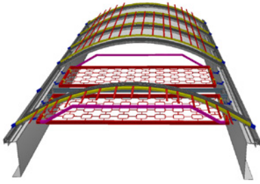
JET continuous rooflight with SHEV full flap permanently and fully effective protection ensured by JET VARIO-SAFEGUARD and JET LB-DDS
