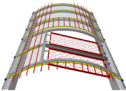
JET continuous rooflight with SHEV lateral flap permanently and fully effective protection ensured by JET VARIO-SAFEGUARD and JET LB-DDS
