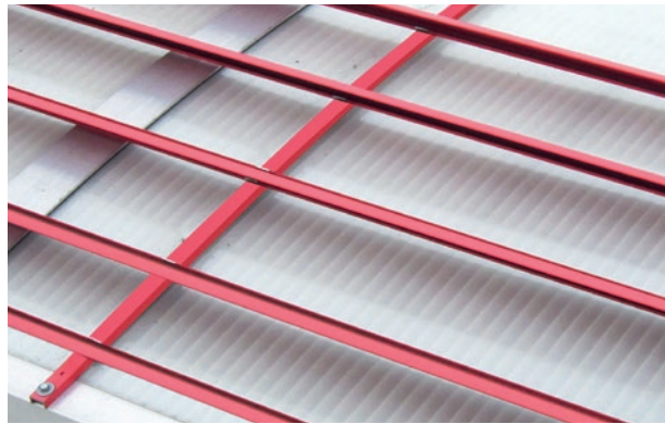
JET VARIO-PROTECT 120 VWS (Traffic route securing) on arched continuous rooflight
